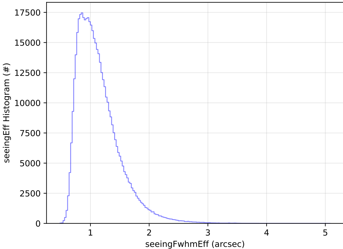
all_long_v3.4_10yrs All sky r band: seeingEff Histogram
