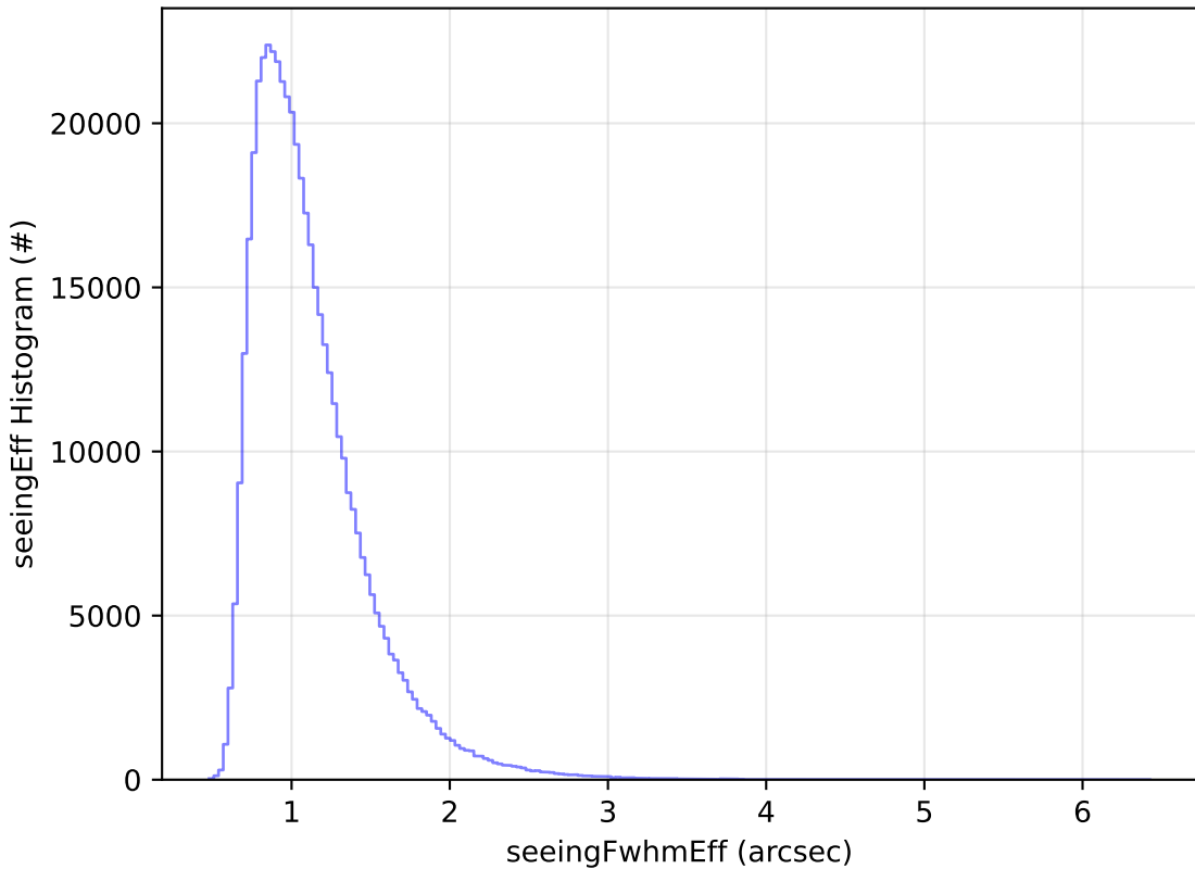
all_long_v3.4_10yrs All sky i band: seeingEff Histogram
