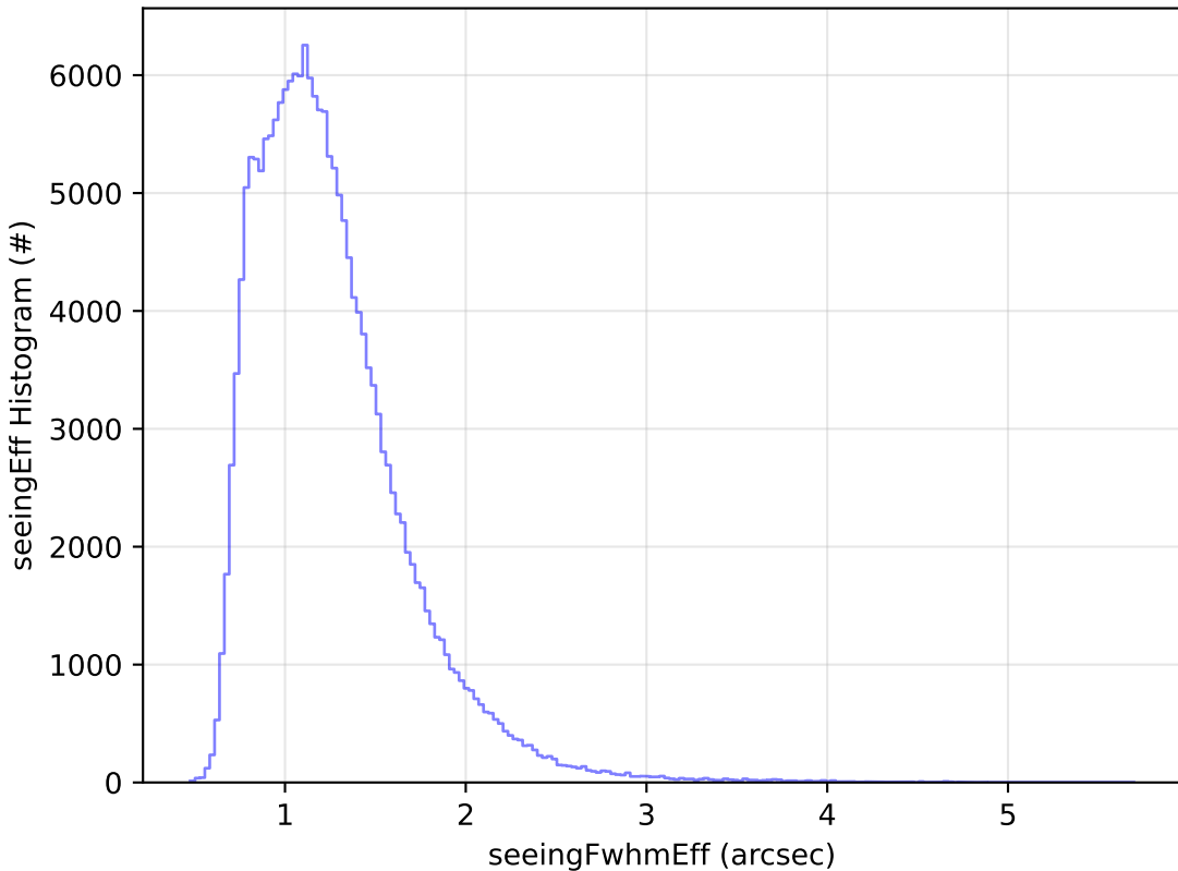
all_long_v3.4_10yrs All sky g band: seeingEff Histogram
