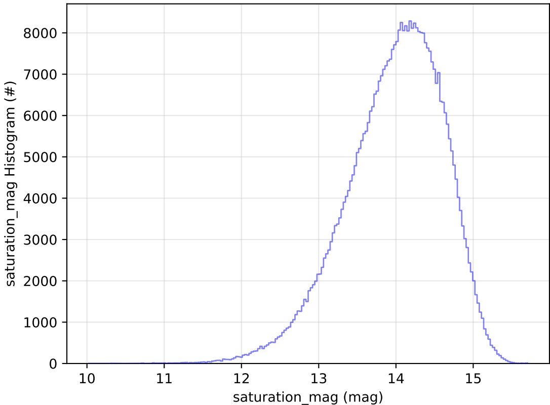
all_long_v3.4_10yrs WFD z band: saturation_mag Histogram
