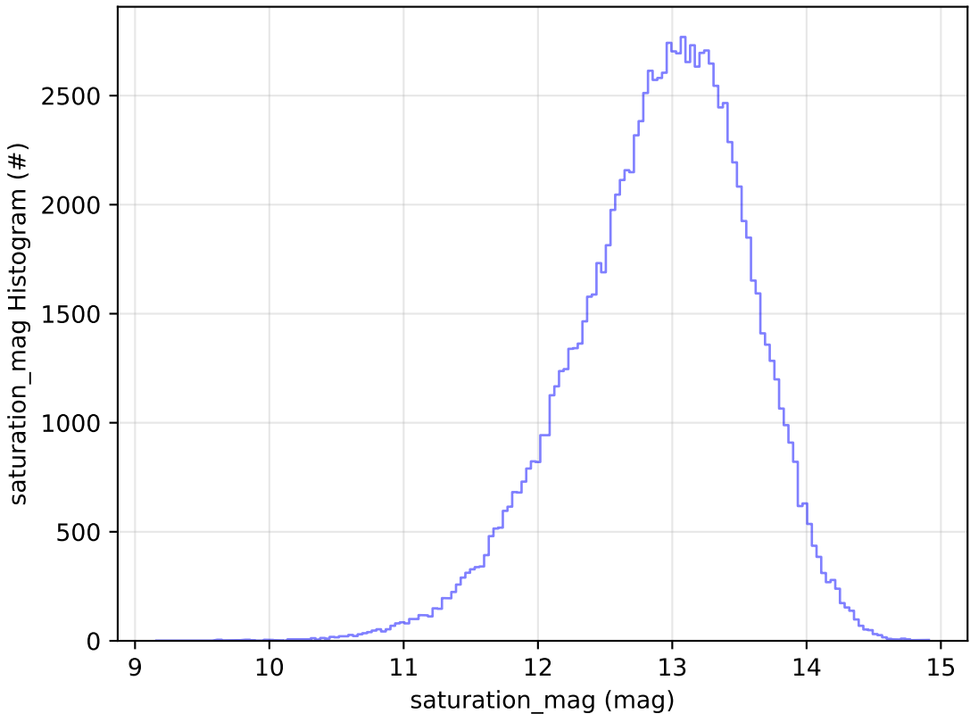
all_long_v3.4_10yrs WFD u band: saturation_mag Histogram
