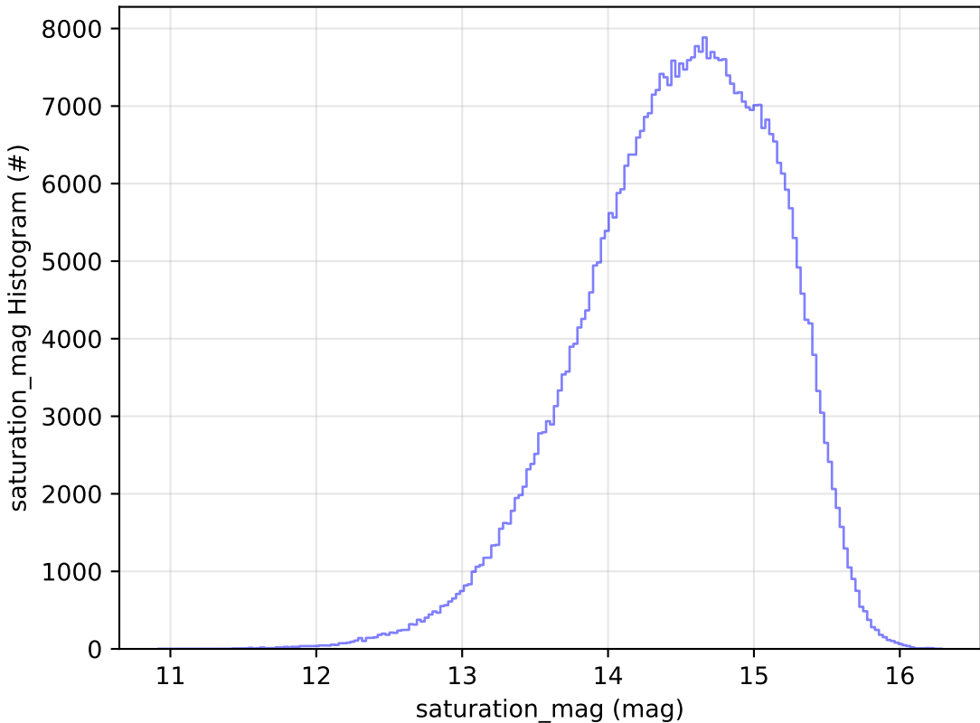
all_long_v3.4_10yrs WFD r band: saturation_mag Histogram
