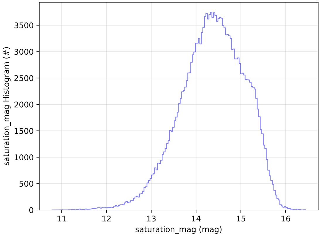
all_long_v3.4_10yrs WFD g band: saturation_mag Histogram
