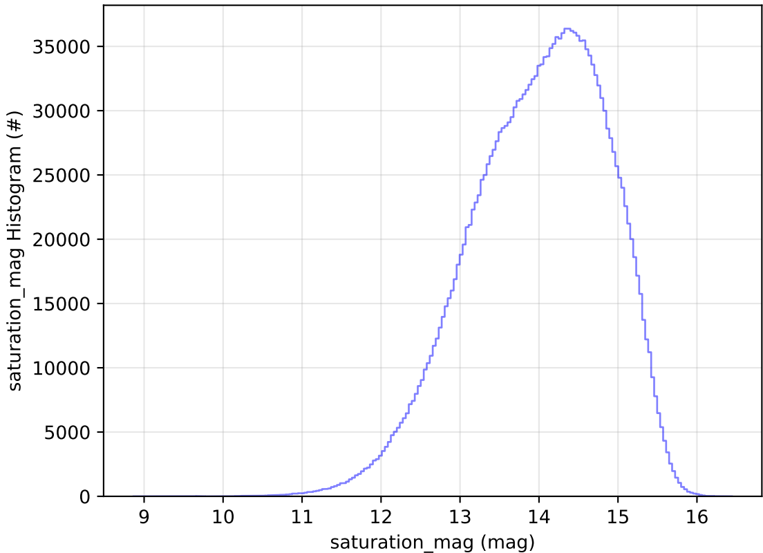
all_long_v3.4_10yrs WFD all bands: saturation_mag Histogram
