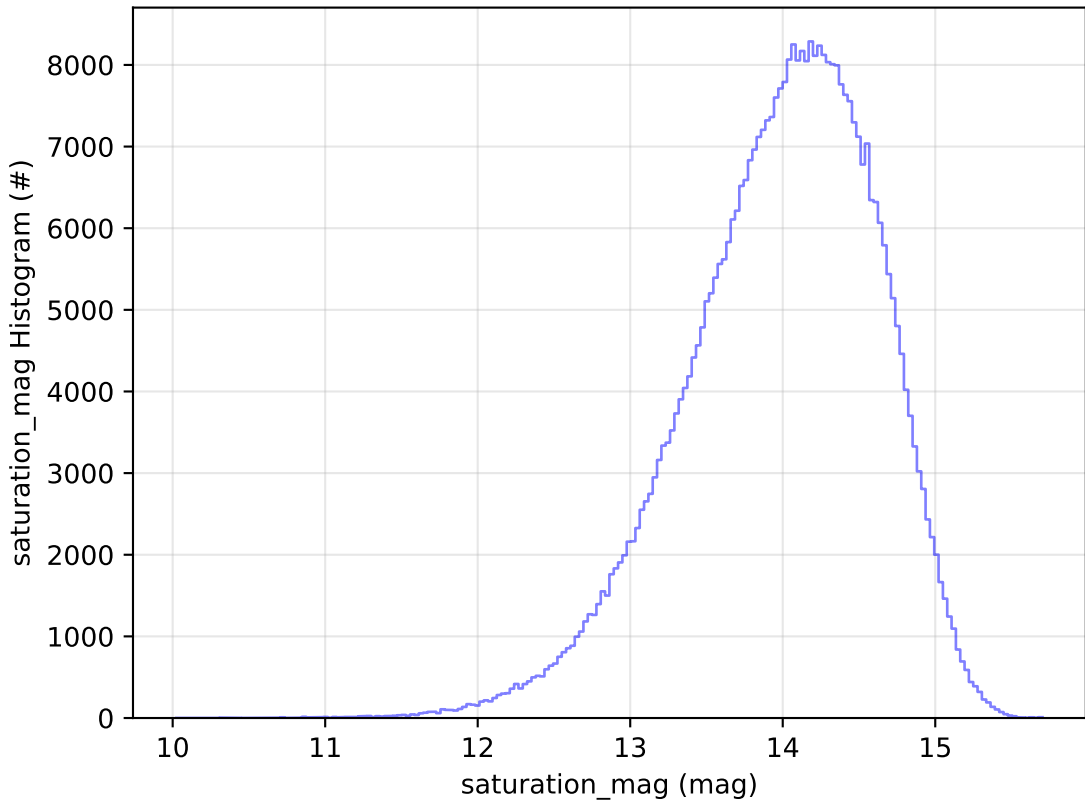
all_long_v3.4_10yrs All sky z band: saturation_mag Histogram
