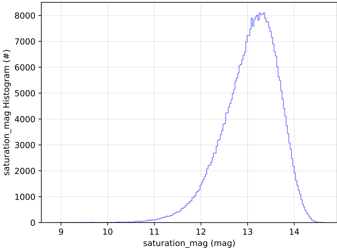
all_long_v3.4_10yrs All sky y band: saturation_mag Histogram
