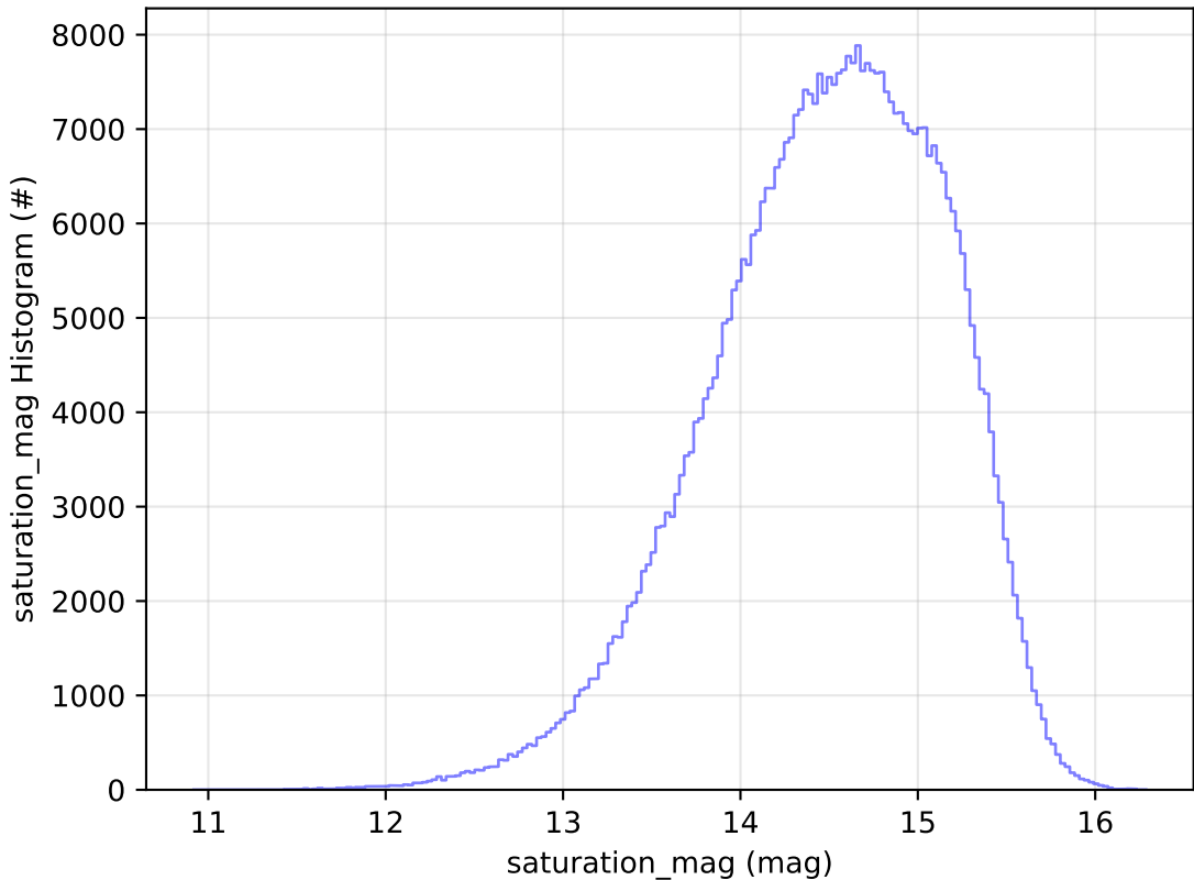
all_long_v3.4_10yrs All sky r band: saturation_mag Histogram
