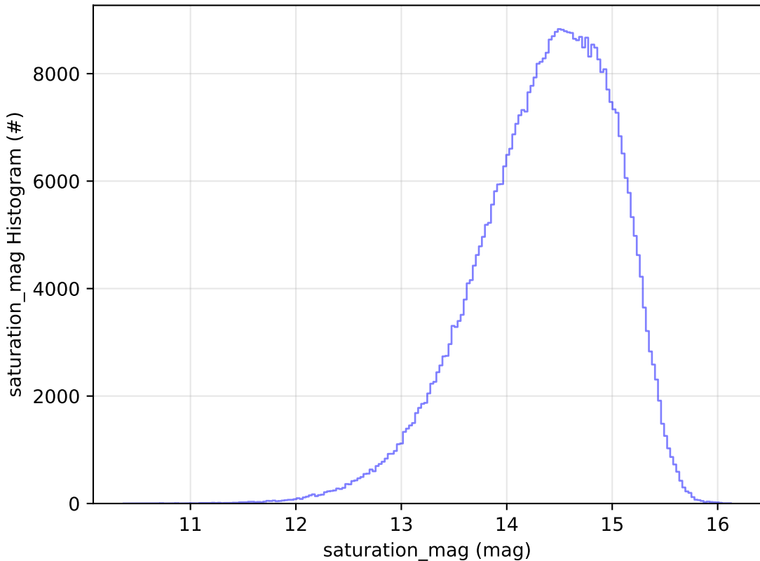
all_long_v3.4_10yrs All sky i band: saturation_mag Histogram
