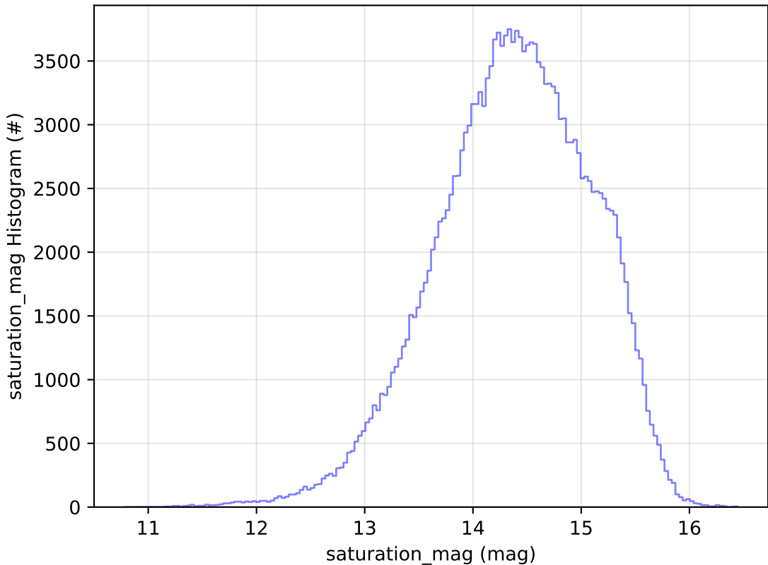
all_long_v3.4_10yrs All sky g band: saturation_mag Histogram
