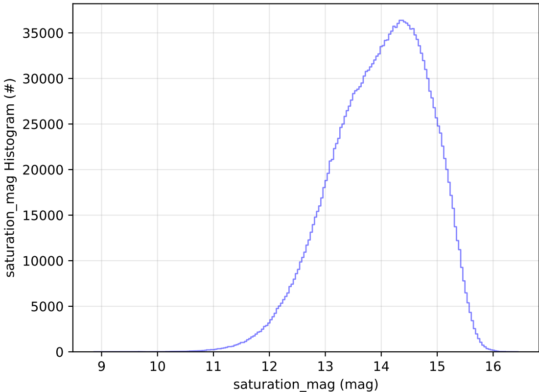
all_long_v3.4_10yrs All sky all bands: saturation_mag Histogram
