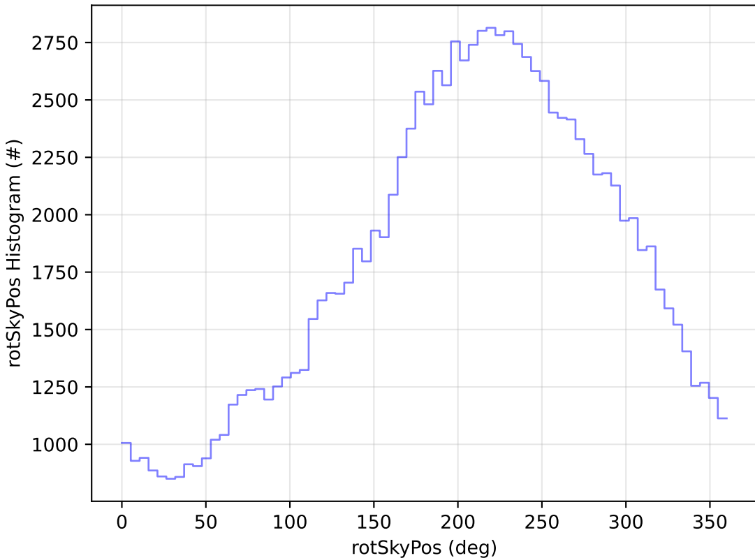
all_long_v3.4_10yrs WFD u band: rotSkyPos Histogram
