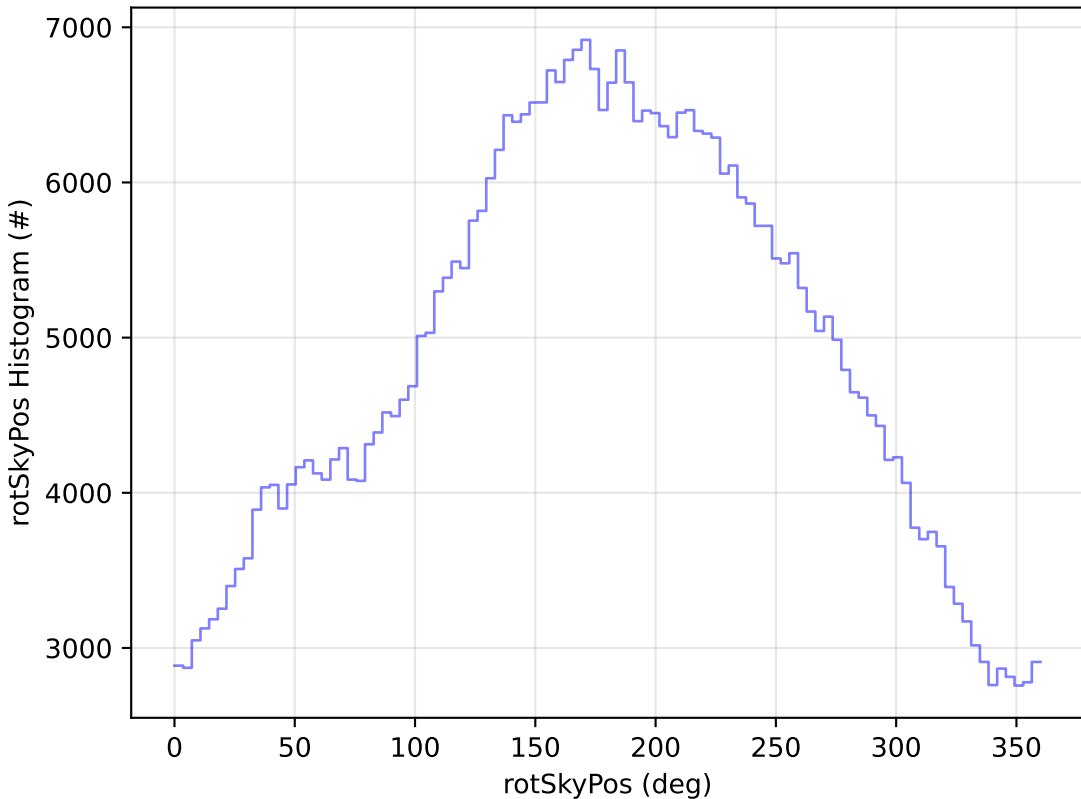
all_long_v3.4_10yrs WFD r band: rotSkyPos Histogram
