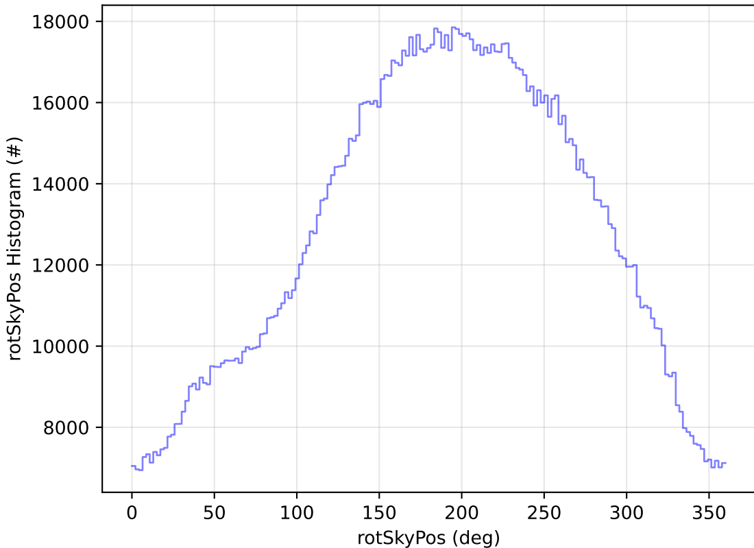
all_long_v3.4_10yrs All sky all bands: rotSkyPos Histogram
