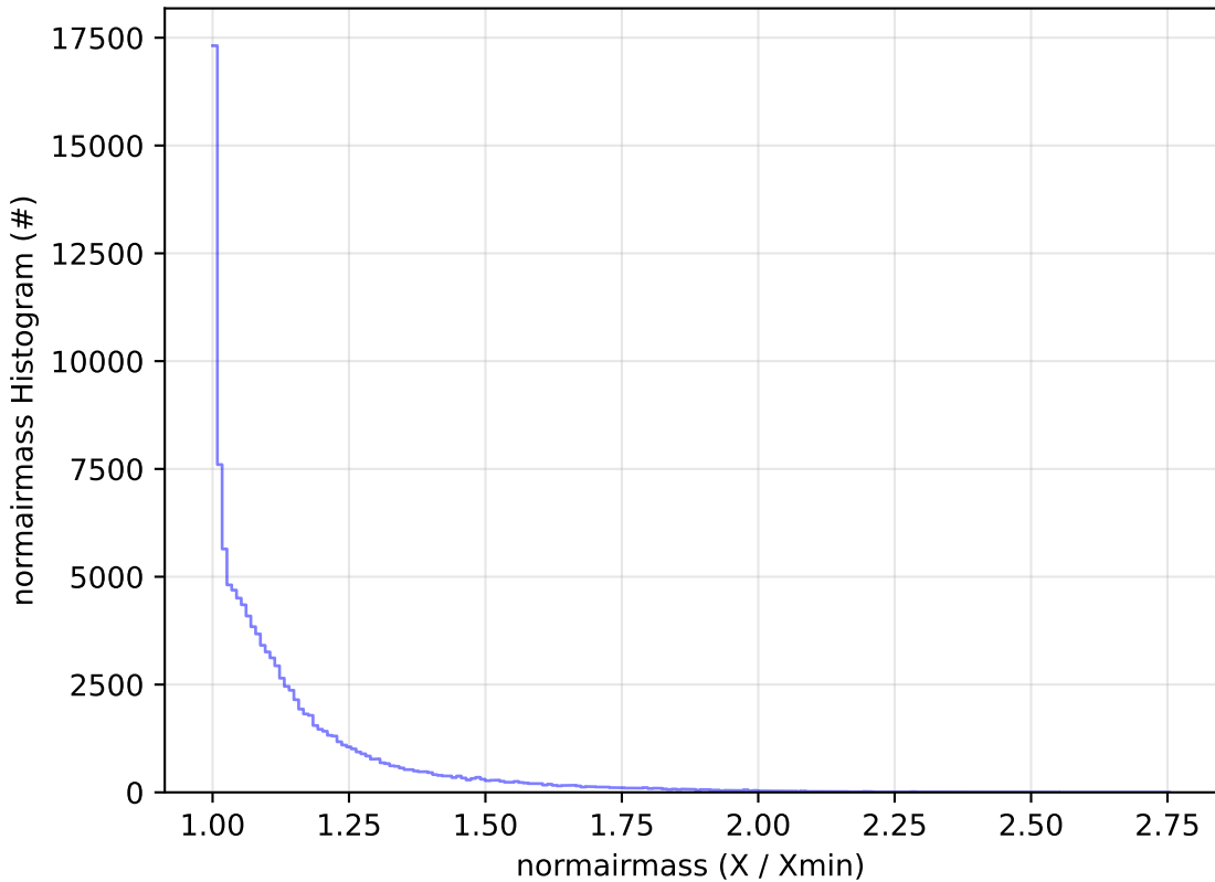
all_long_v3.4_10yrs WFD u band: normairmass Histogram
