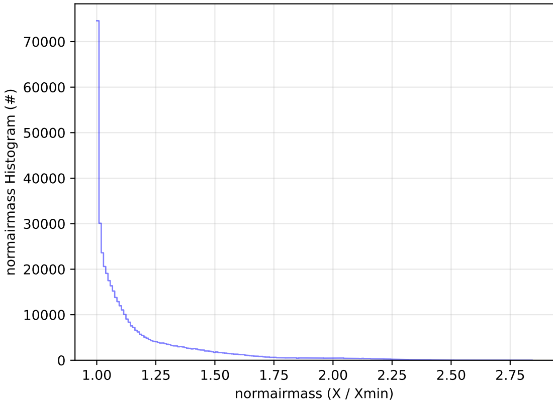
all_long_v3.4_10yrs WFD r band: normairmass Histogram
