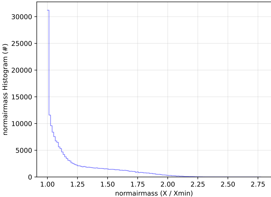
all_long_v3.4_10yrs WFD g band: normairmass Histogram
