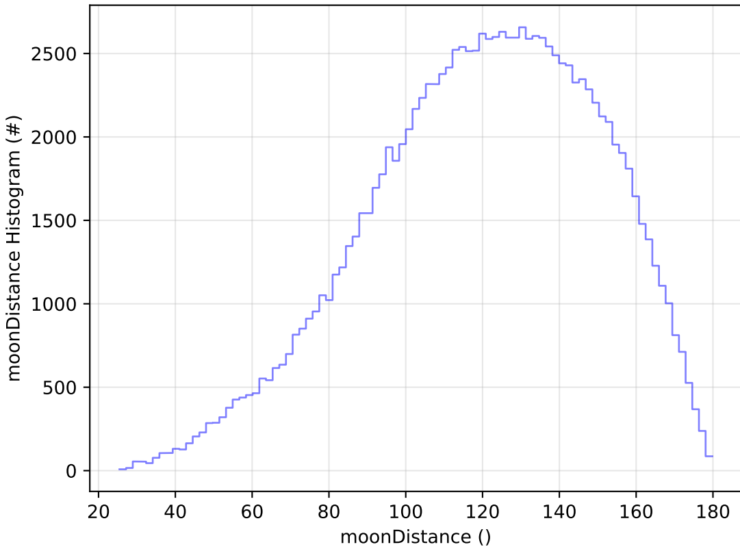
all_long_v3.4_10yrs WFD u band: moonDistance Histogram
