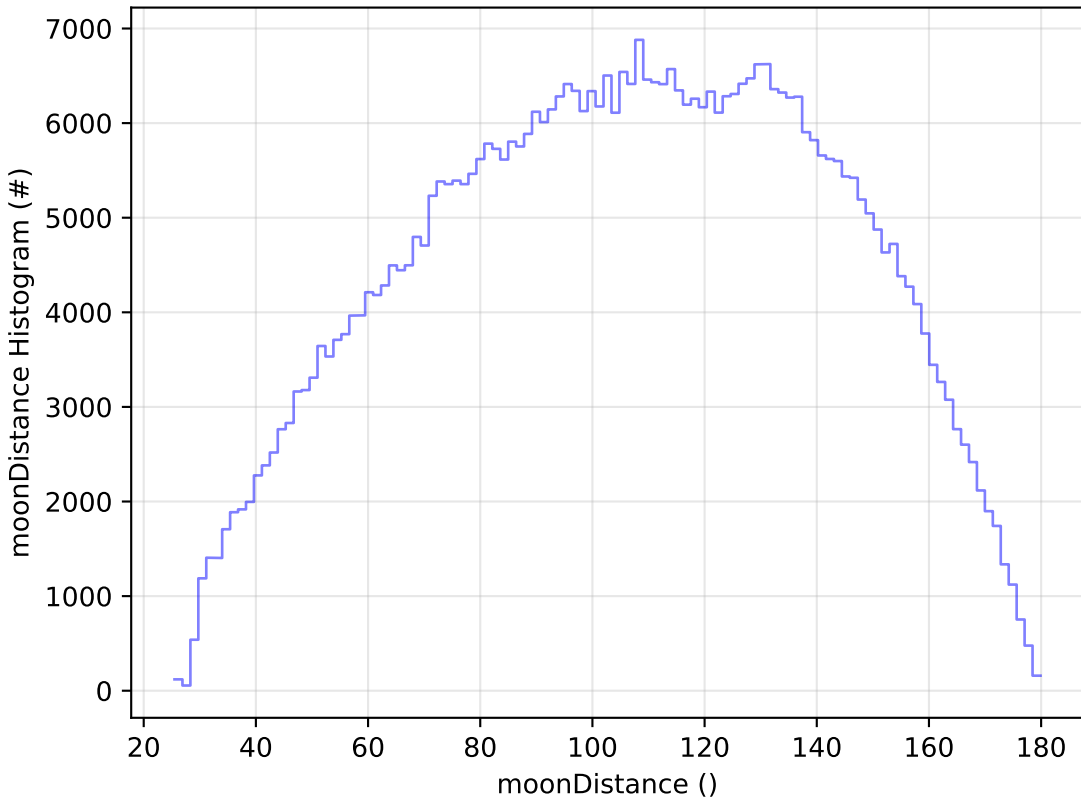
all_long_v3.4_10yrs WFD r band: moonDistance Histogram
