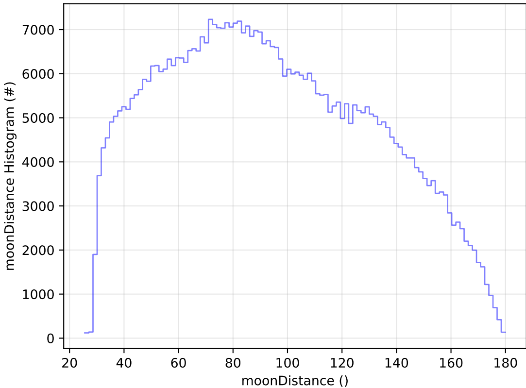
all_long_v3.4_10yrs WFD i band: moonDistance Histogram
