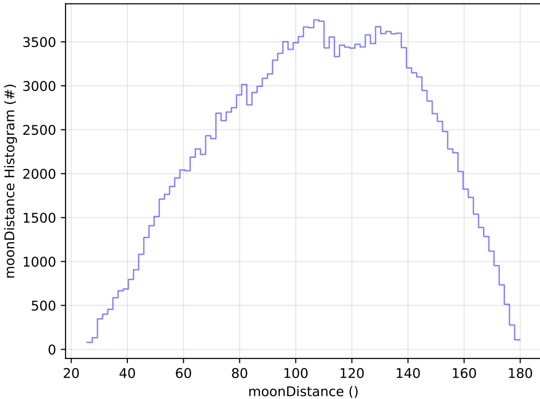
all_long_v3.4_10yrs WFD g band: moonDistance Histogram
