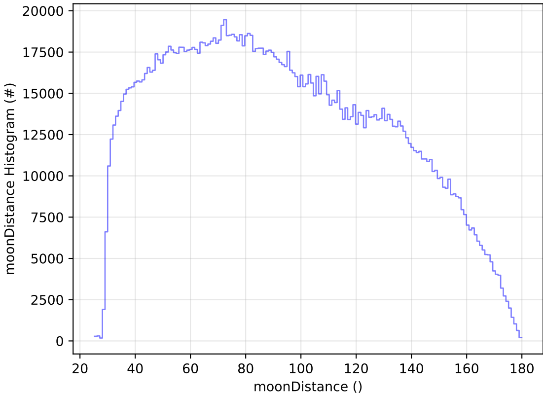
all_long_v3.4_10yrs WFD all bands: moonDistance Histogram
