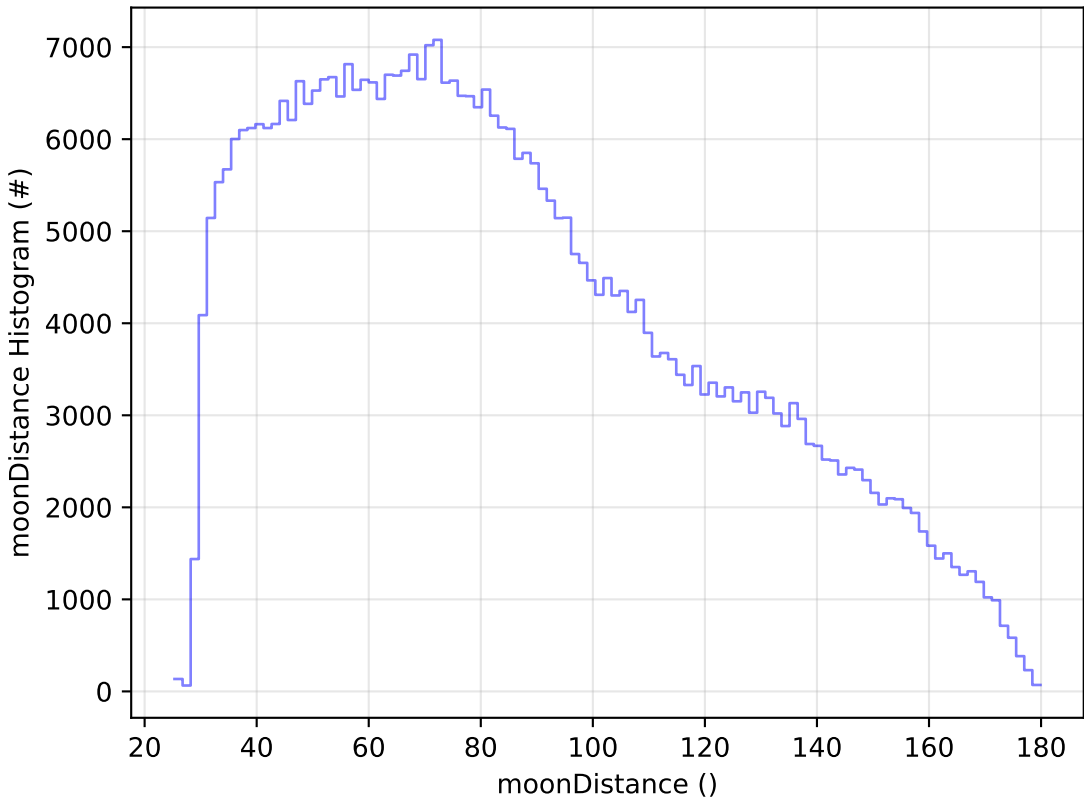
all_long_v3.4_10yrs All sky z band: moonDistance Histogram
