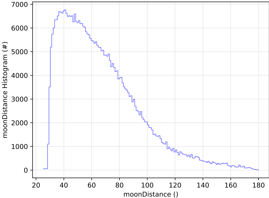
all_long_v3.4_10yrs All sky y band: moonDistance Histogram
