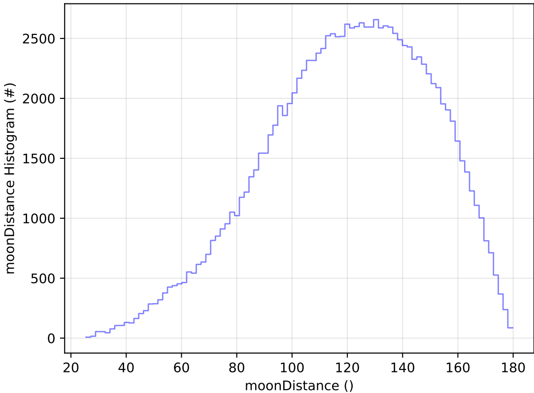
all_long_v3.4_10yrs All sky u band: moonDistance Histogram
