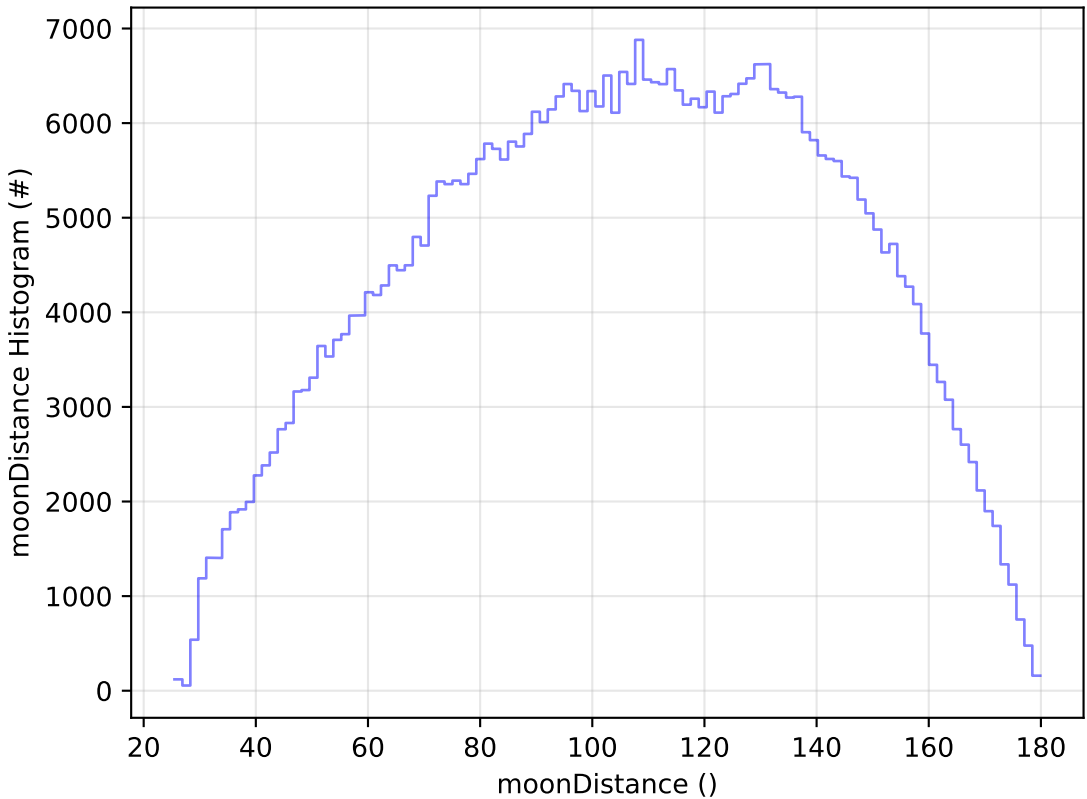
all_long_v3.4_10yrs All sky r band: moonDistance Histogram
