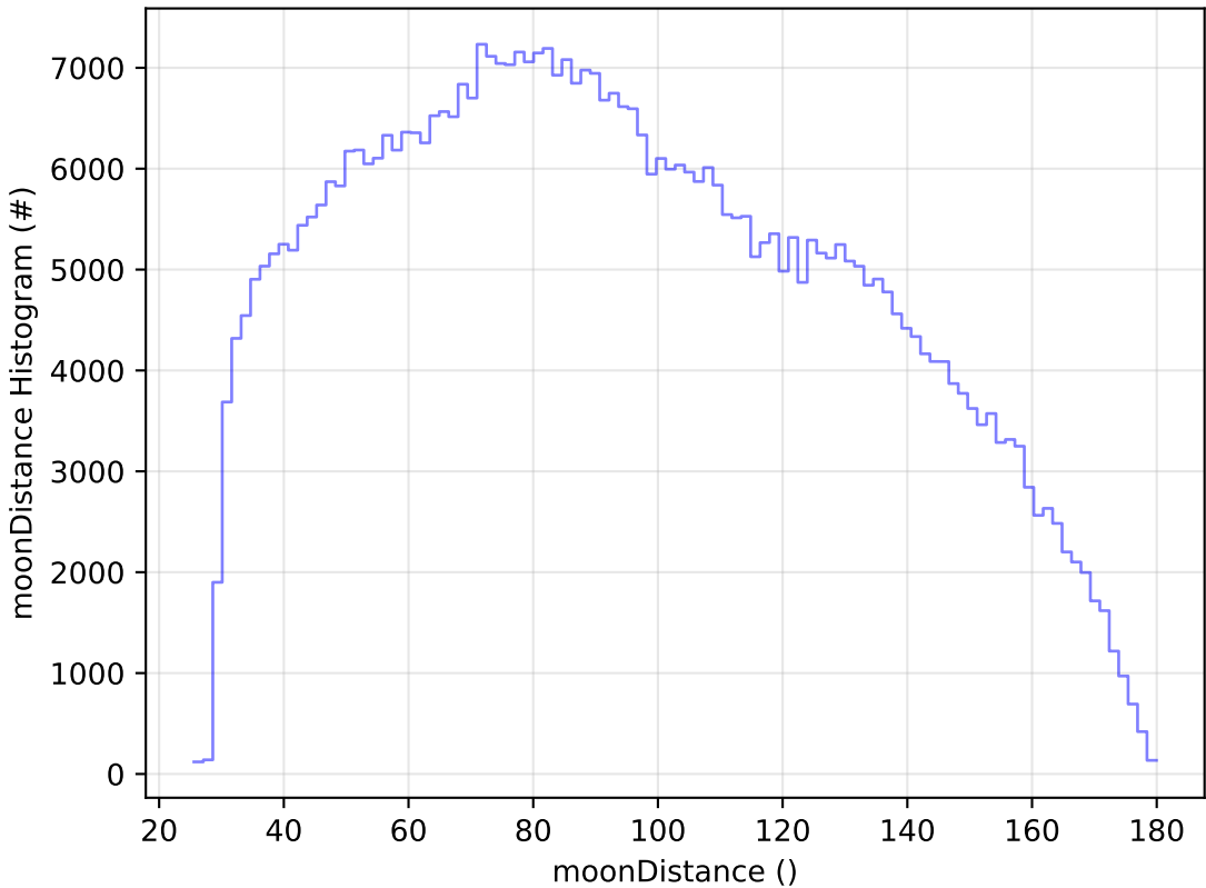
all_long_v3.4_10yrs All sky i band: moonDistance Histogram
