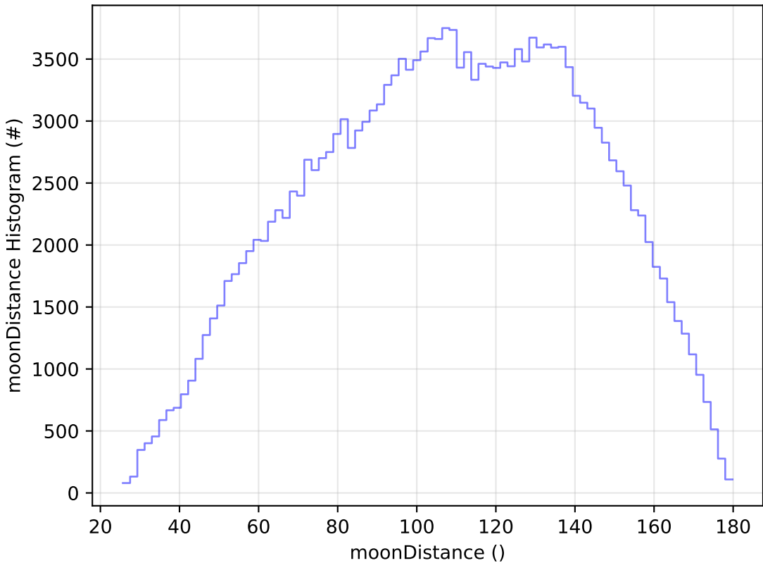
all_long_v3.4_10yrs All sky g band: moonDistance Histogram
