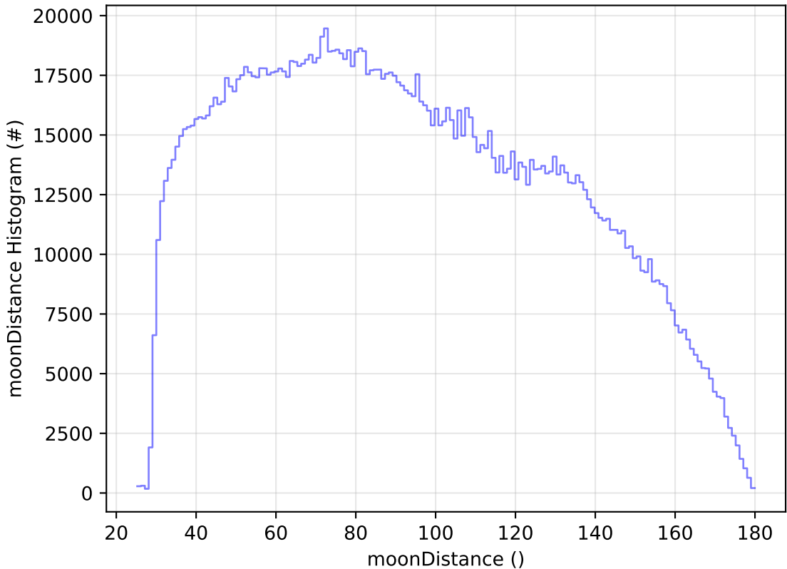
all_long_v3.4_10yrs All sky all bands: moonDistance Histogram
