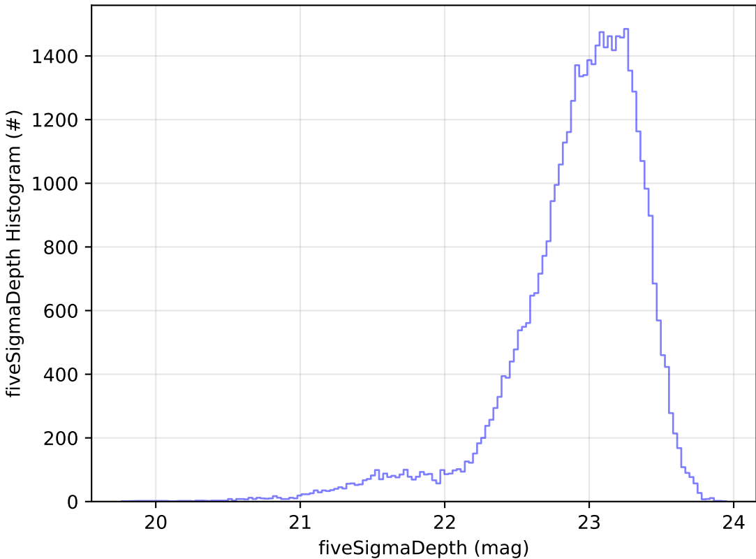
all_long_v3.4_10yrs Yr 1 z band: fiveSigmaDepth Histogram
