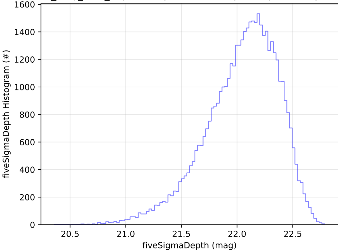
all_long_v3.4_10yrs Yr 1 y band: fiveSigmaDepth Histogram
