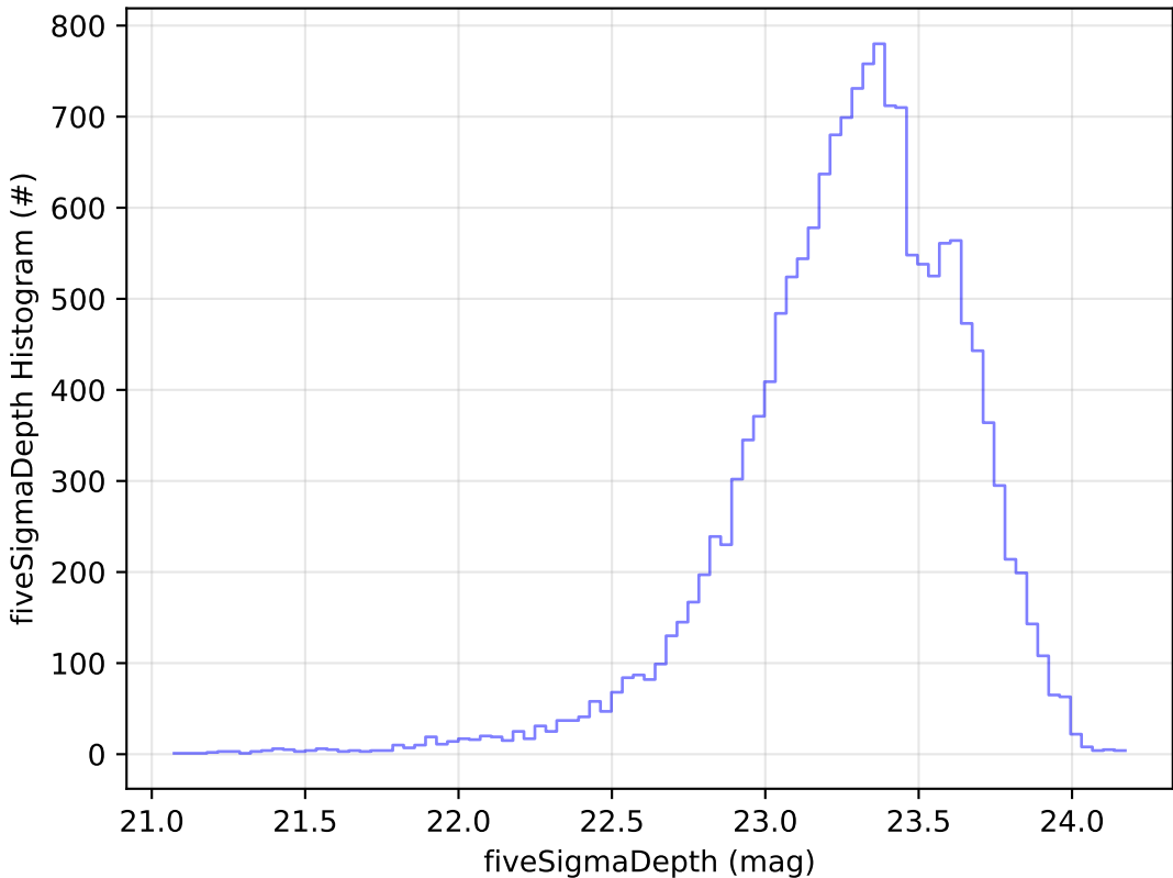
all_long_v3.4_10yrs Yr 1 u band: fiveSigmaDepth Histogram
