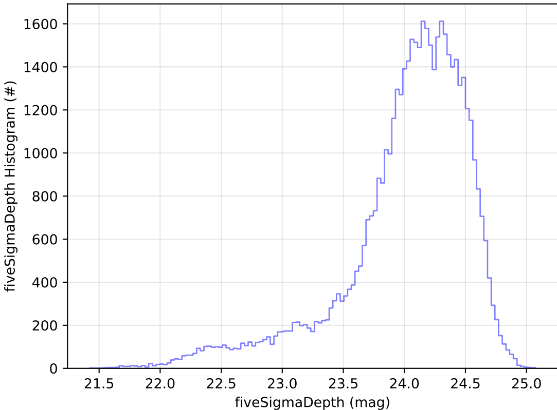
all_long_v3.4_10yrs Yr 1 r band: fiveSigmaDepth Histogram
