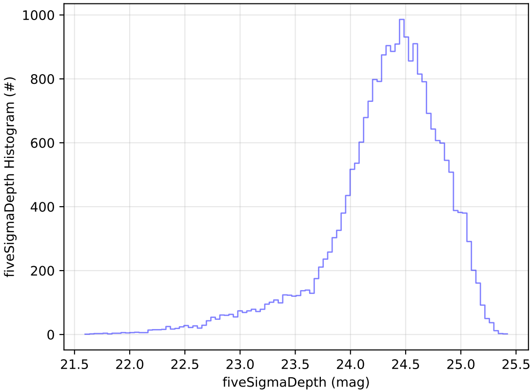
all_long_v3.4_10yrs Yr 1 g band: fiveSigmaDepth Histogram
