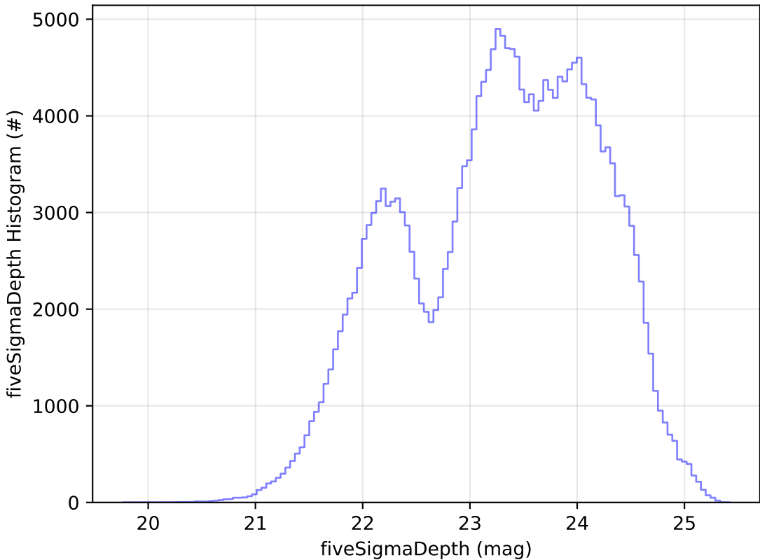
all_long_v3.4_10yrs Yr 1 all bands: fiveSigmaDepth Histogram
