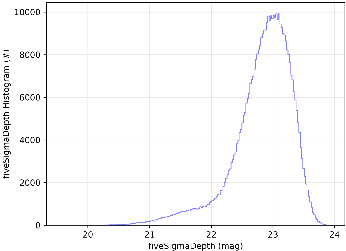
all_long_v3.4_10yrs WFD z band: fiveSigmaDepth Histogram
