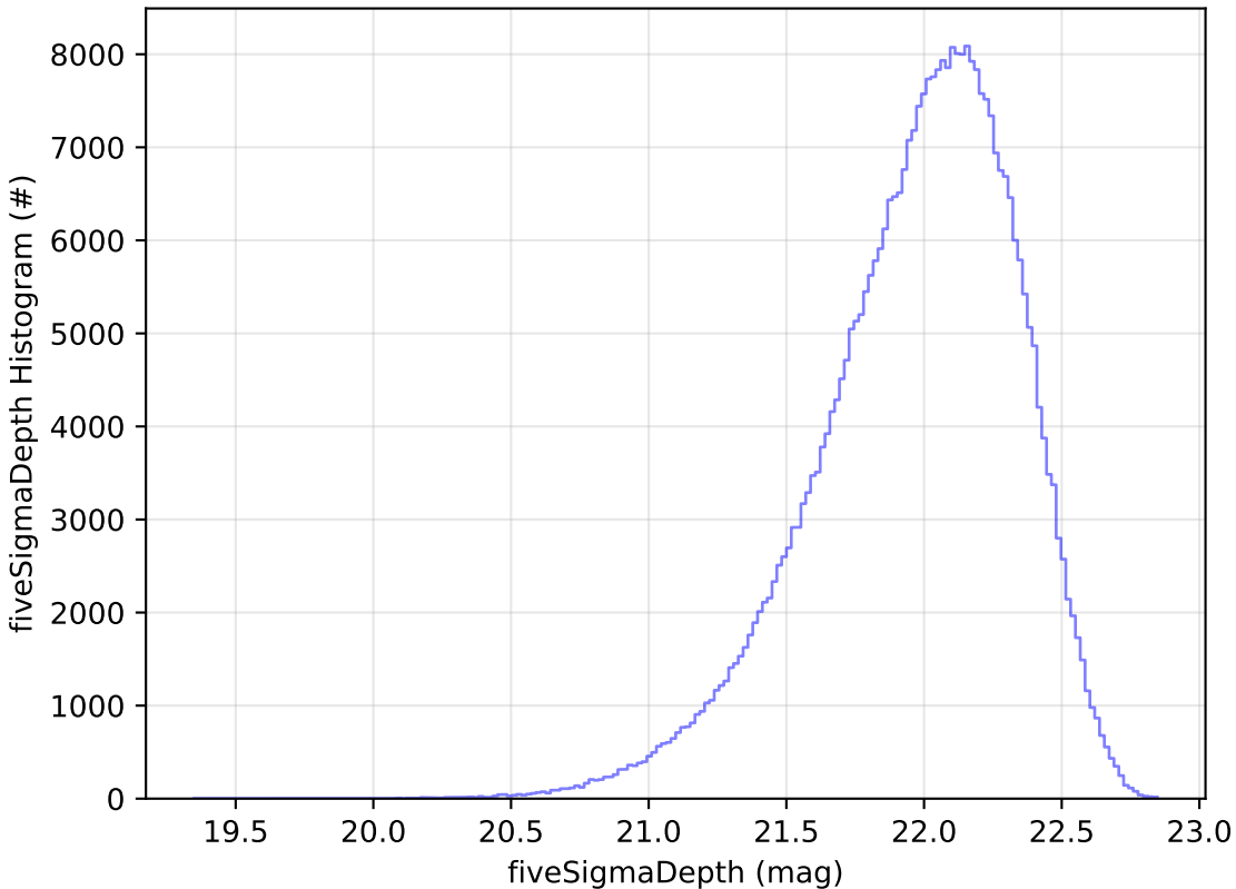
all_long_v3.4_10yrs WFD y band: fiveSigmaDepth Histogram
