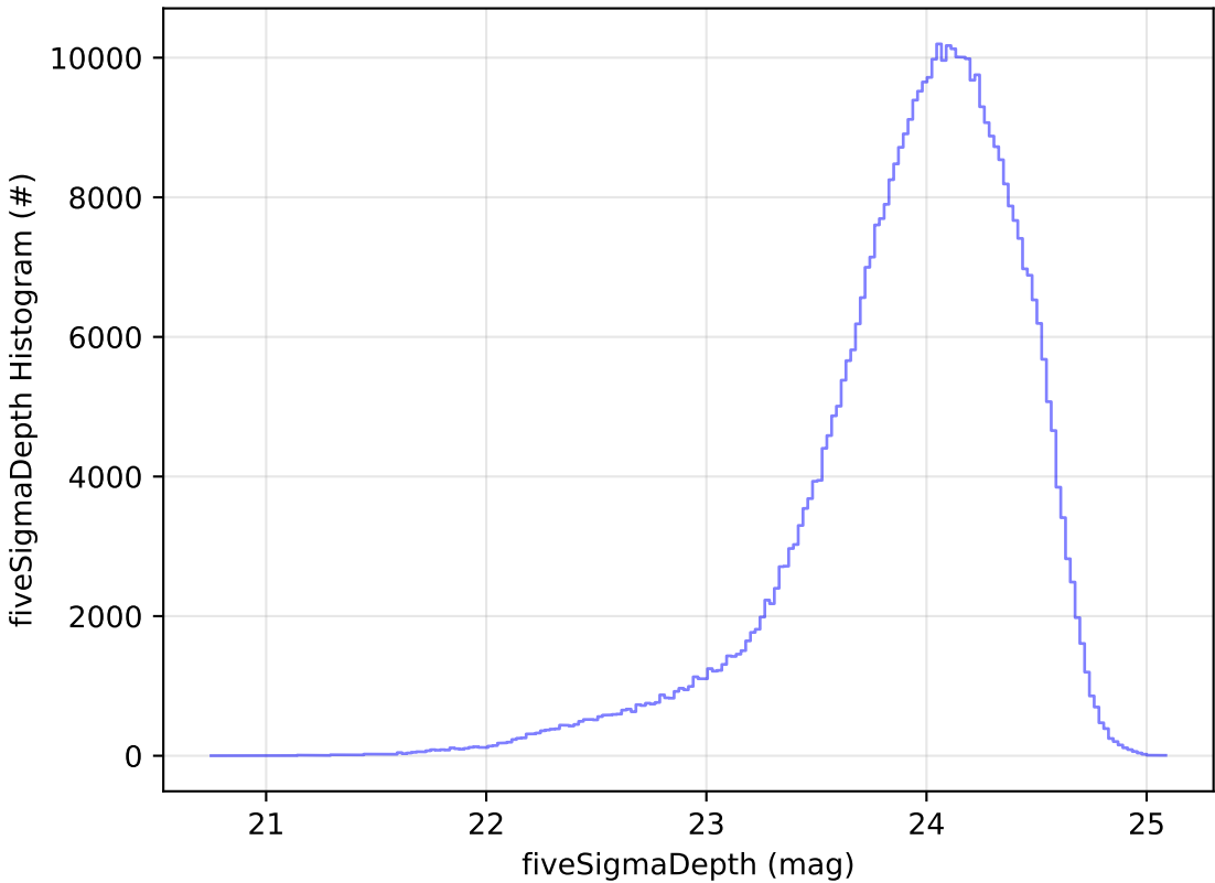
all_long_v3.4_10yrs WFD r band: fiveSigmaDepth Histogram
