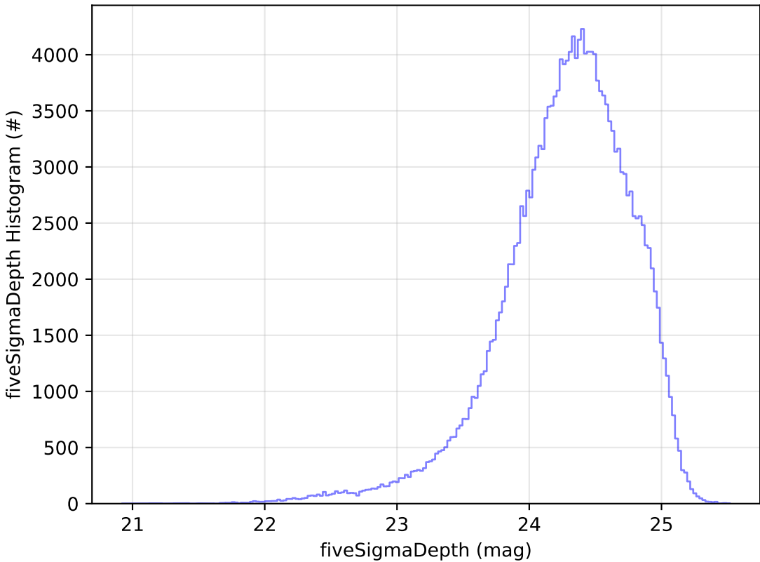
all_long_v3.4_10yrs WFD g band: fiveSigmaDepth Histogram
