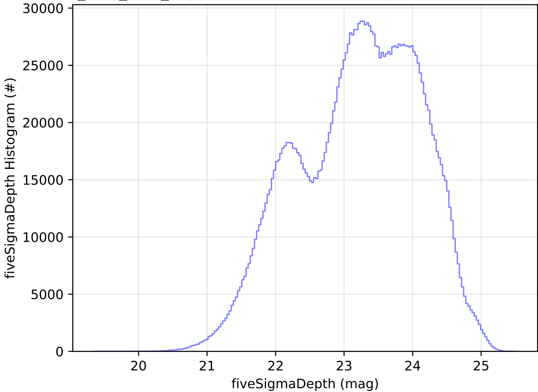
all_long_v3.4_10yrs WFD all bands: fiveSigmaDepth Histogram
