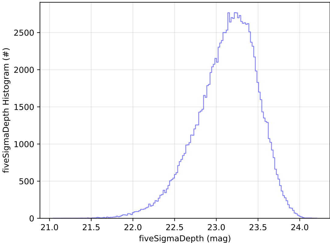
all_long_v3.4_10yrs All sky u band: fiveSigmaDepth Histogram
