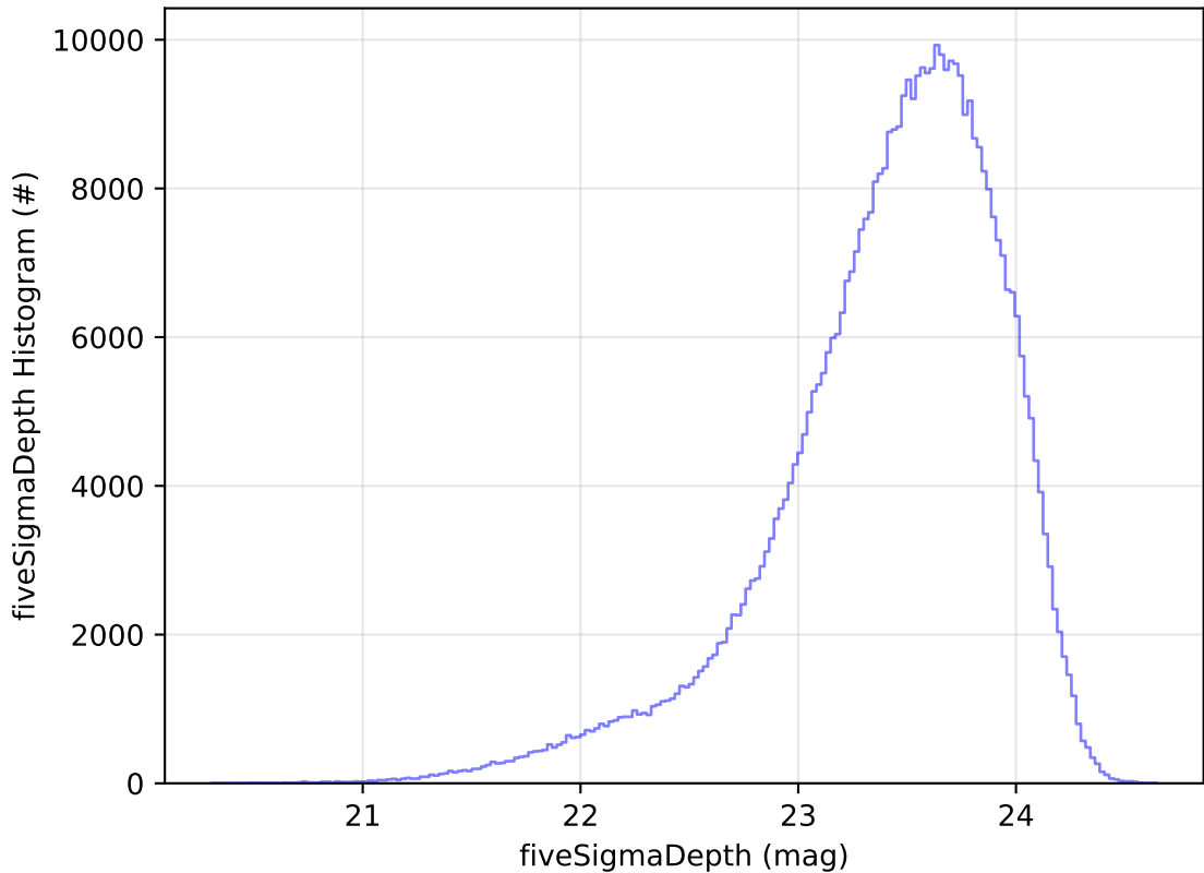
all_long_v3.4_10yrs All sky i band: fiveSigmaDepth Histogram
