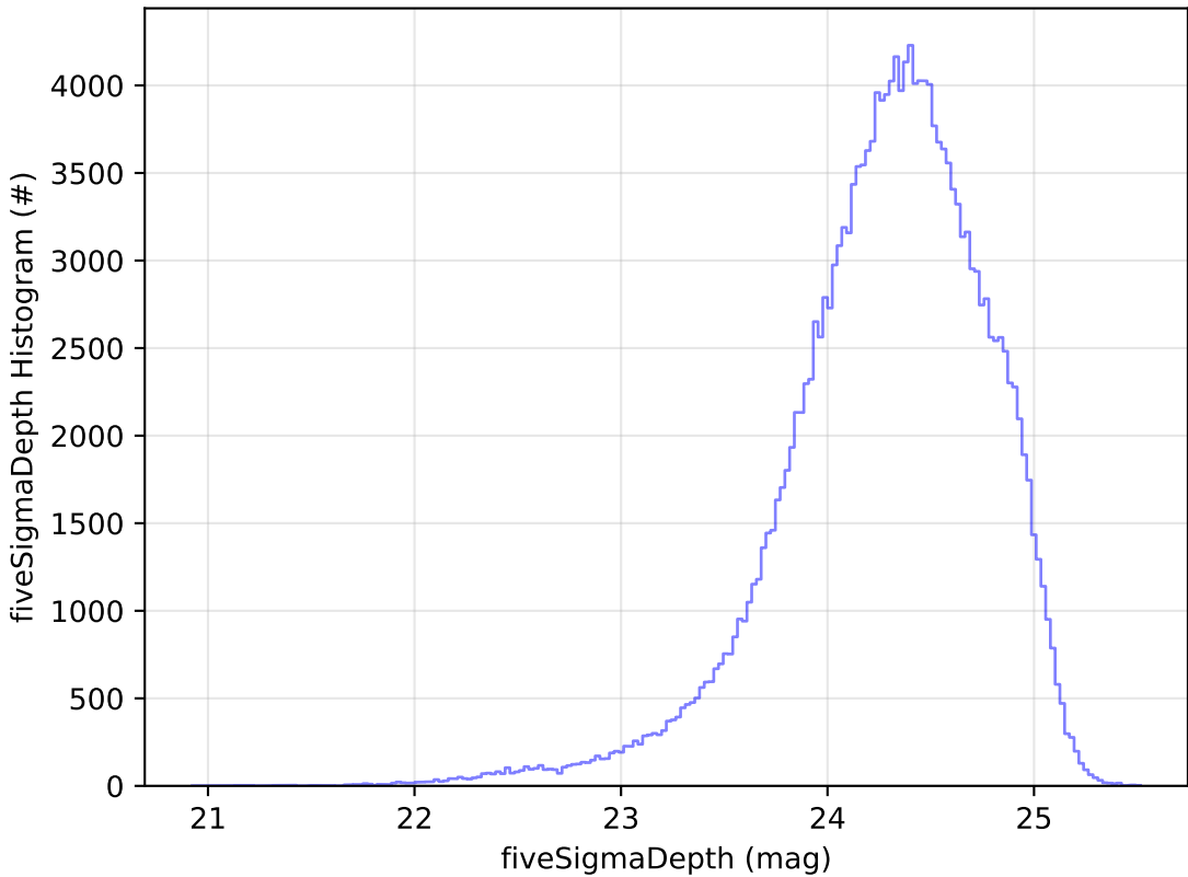
all_long_v3.4_10yrs All sky g band: fiveSigmaDepth Histogram
