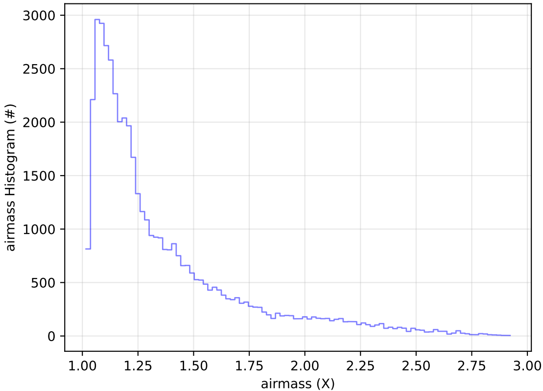
all_long_v3.4_10yrs Yr 1 z band: airmass Histogram
