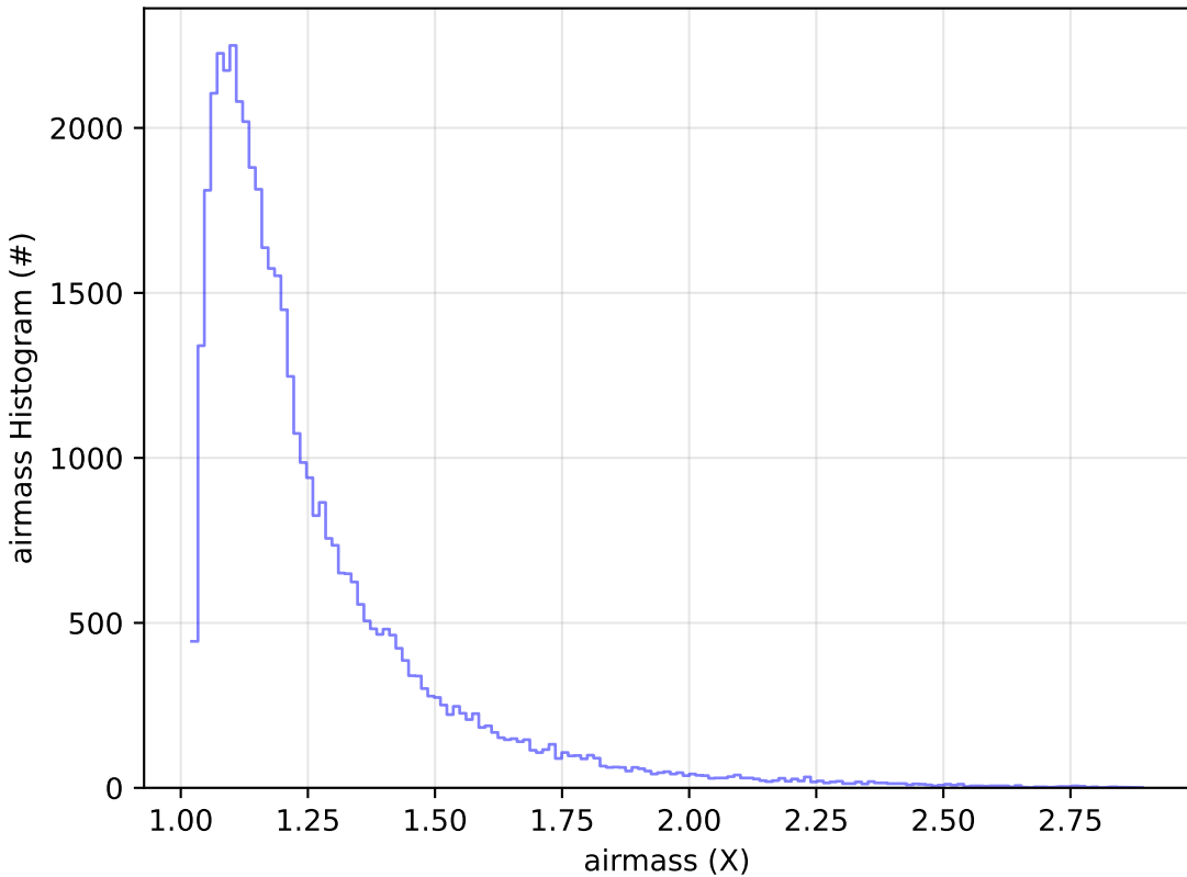
all_long_v3.4_10yrs Yr 1 y band: airmass Histogram
