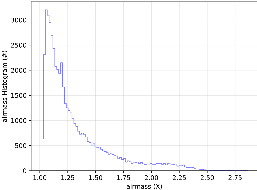
all_long_v3.4_10yrs Yr 1 r band: airmass Histogram
