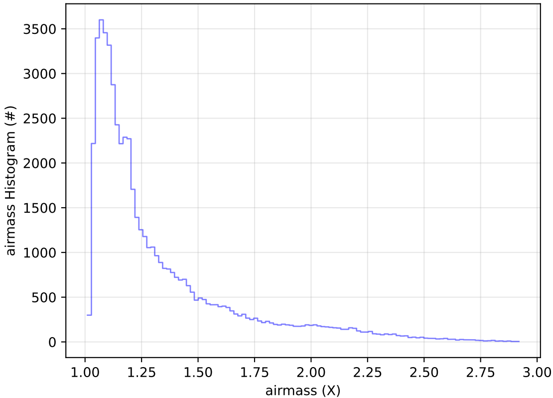
all_long_v3.4_10yrs Yr 1 i band: airmass Histogram
